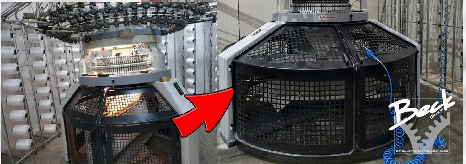
Mayer & Cie OV3.2 30"x 28E Open Width transformed
